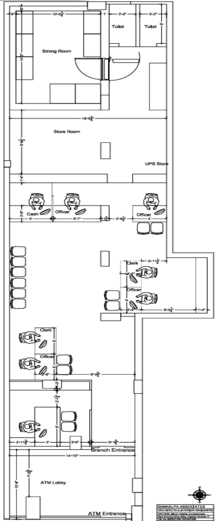
INTERIOR LAYOUT OF PROPOSED PREMISES FOR VASHI BRANCH FOR INDIAN BANK
