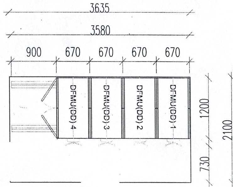
MCB STORE ROOM PLAN LAYOUT DRAWING
