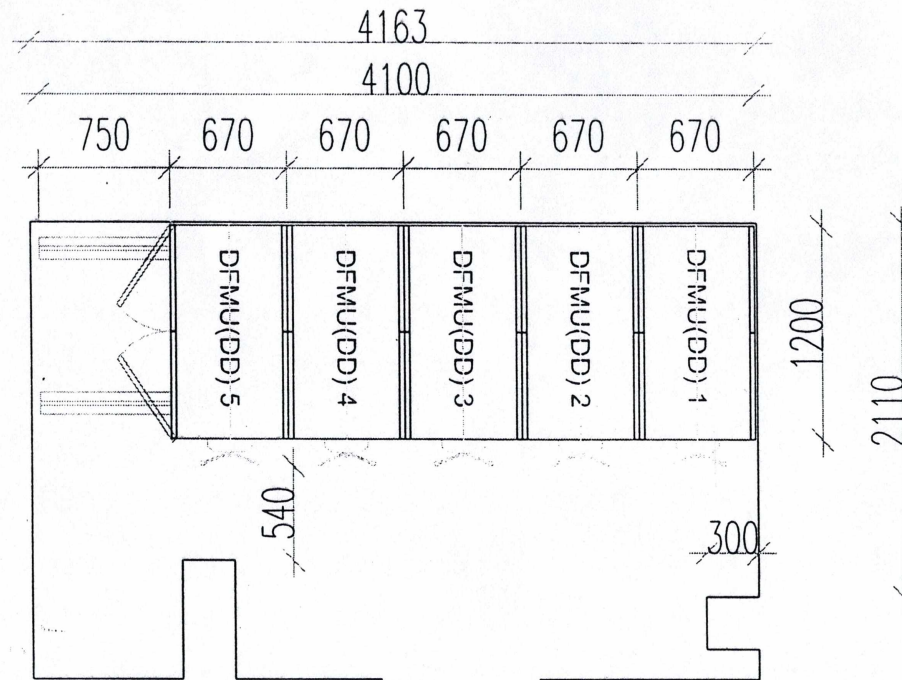
RMPC STORE ROOM PLAN LAYOUT DRAWING
