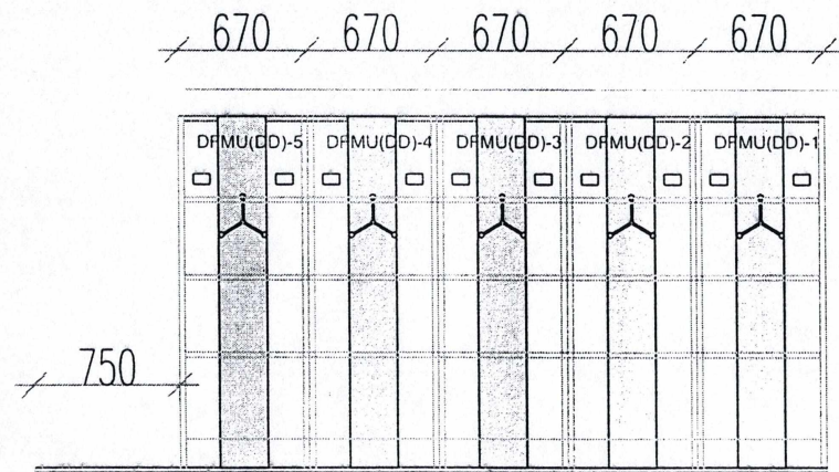
FRONT ELEVATION DRAWING
