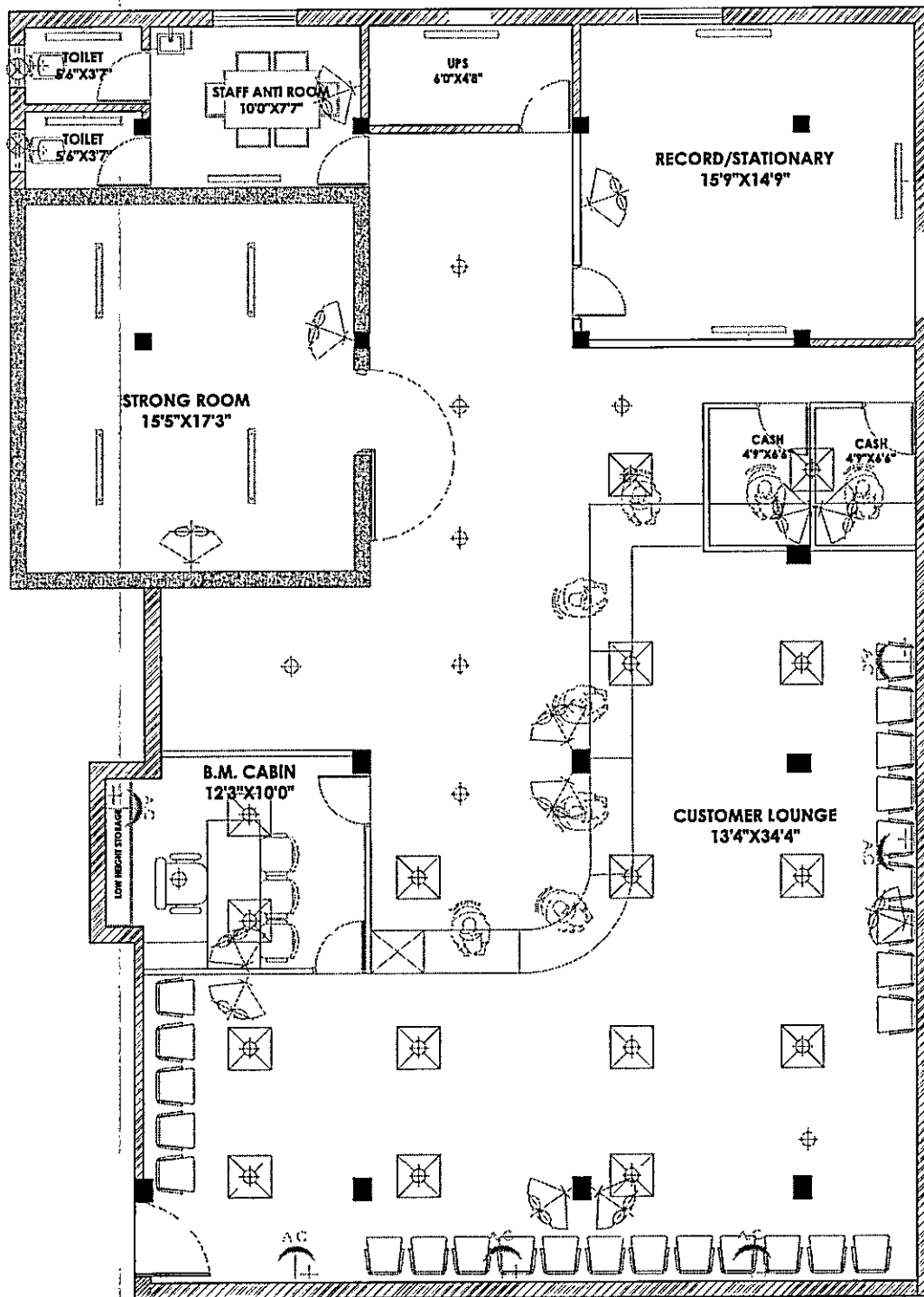
ELECTRICAL FLOOR PLAN-BHEEMAVARAM BRANCH
