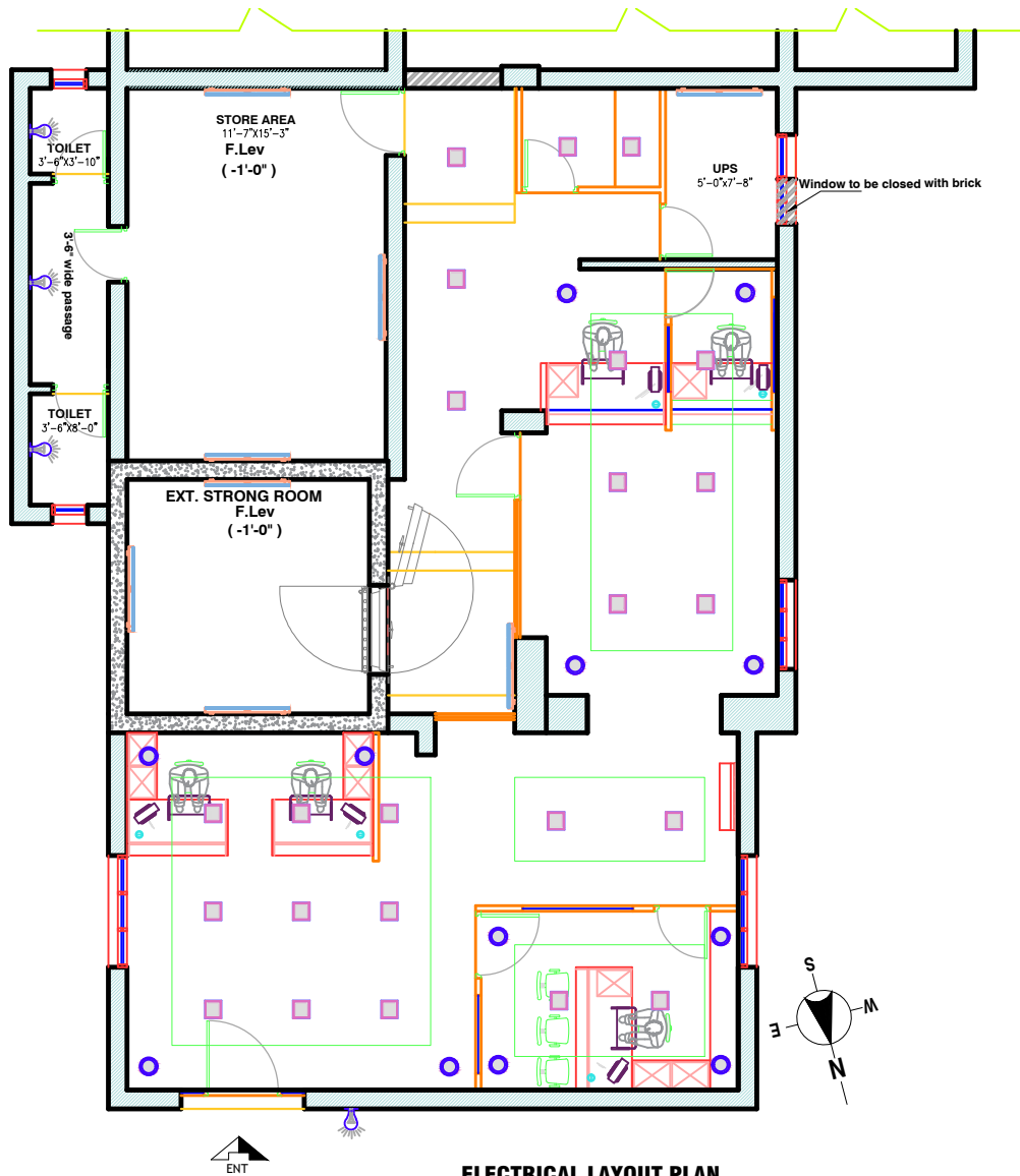
ELECTRICAL LAYOUT PLAN
