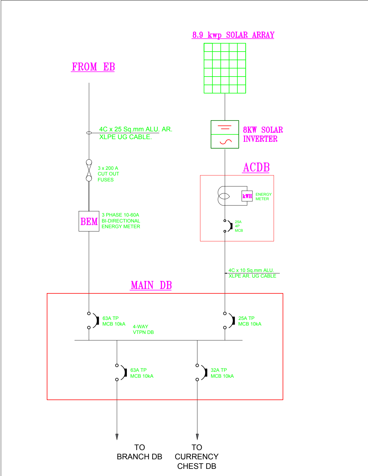
TITLE:- SINGLE LINE DIAGRAM FOR INDIAN BANK, RANIPET BRANCH
