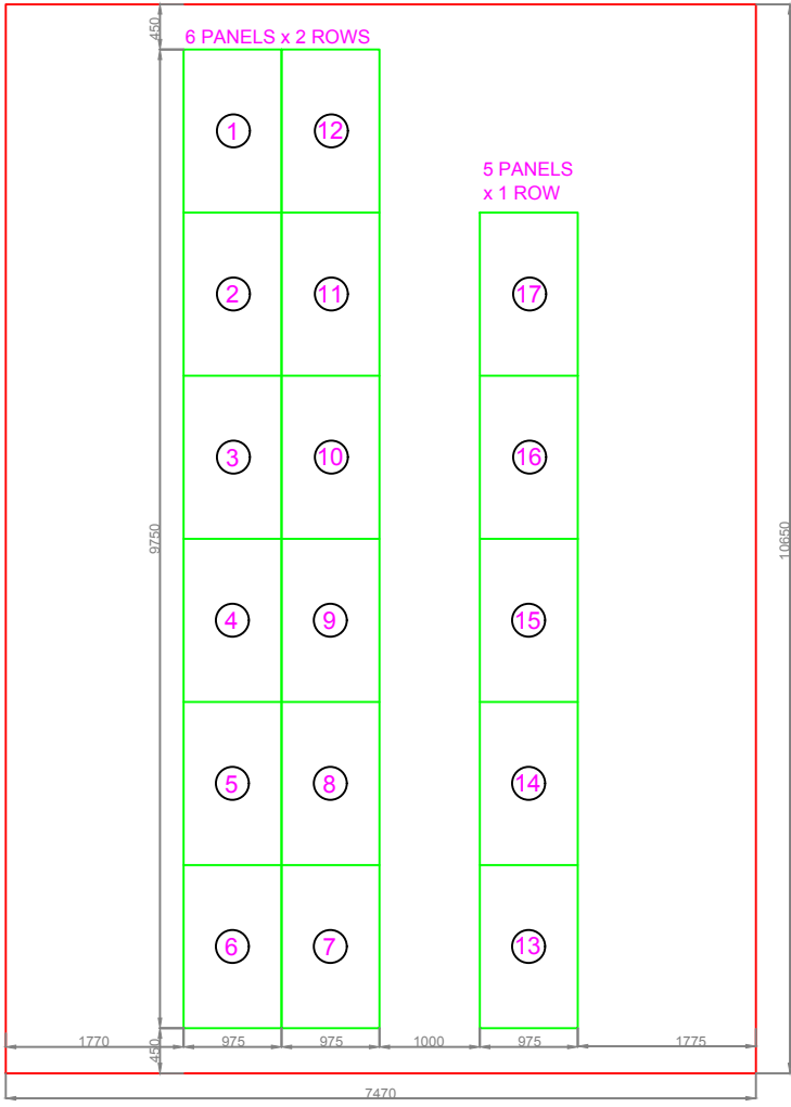
FRONT WING
