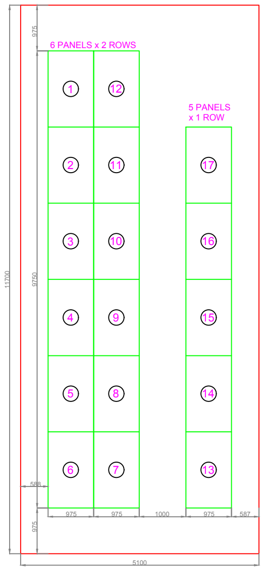
REAR WING
