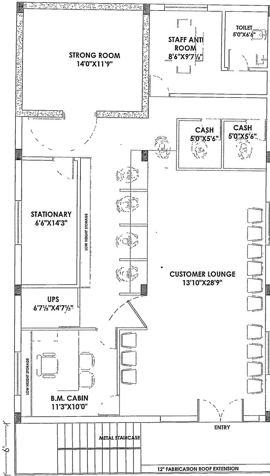
INTERIOR FLOOR PLAN TEKKALI BRANCH
