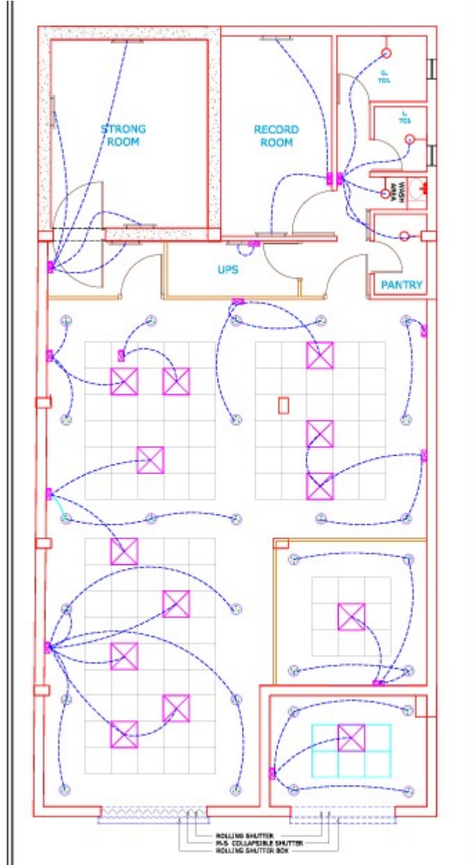
DRAWING : LAYOUT PLAN LIGHT POINTS
