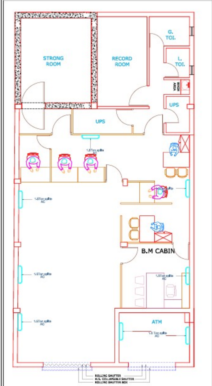
DRAWING : AC POINT LAY OUT PLAN
