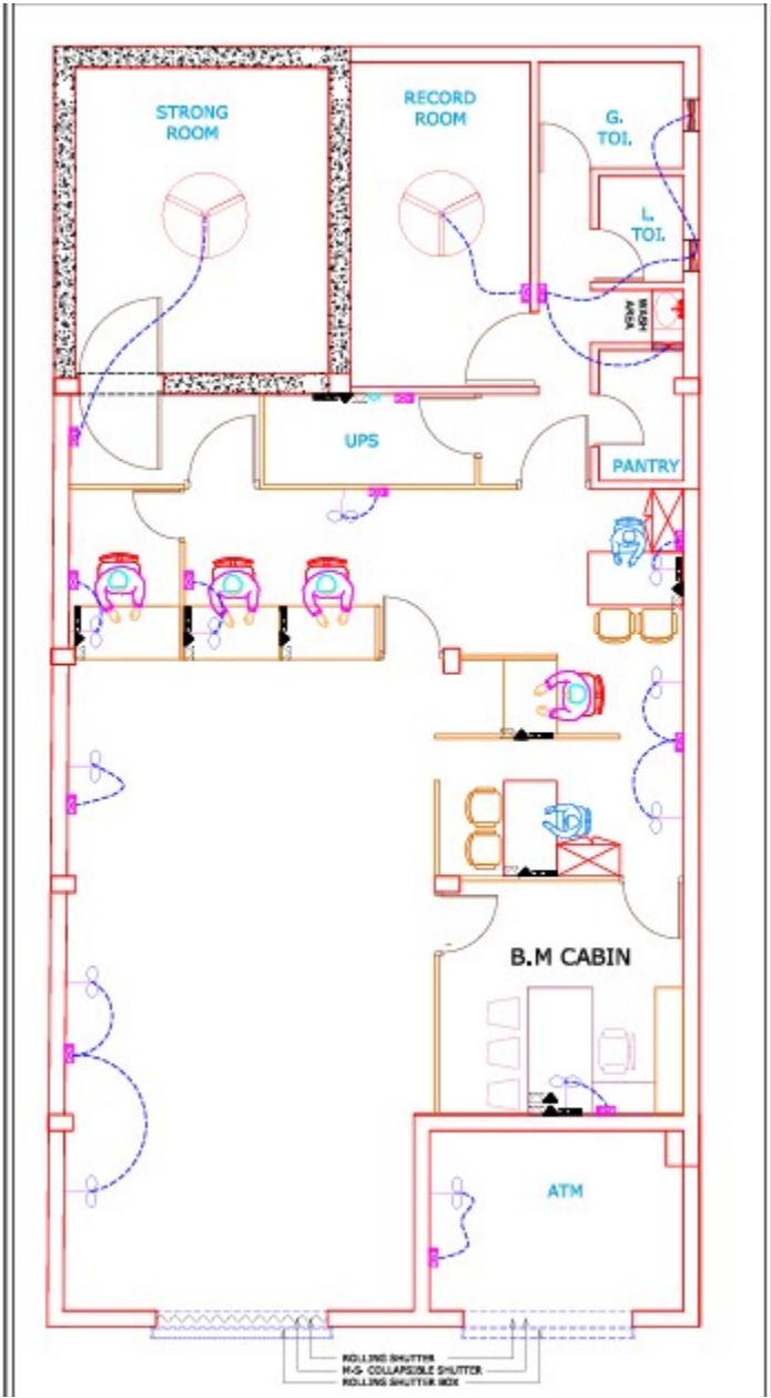
DRAWING : ELECTRICAL PLAN Layout Plan Data & Fan Points
