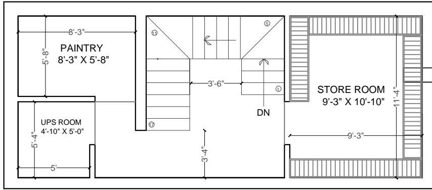
BASEMENT FLOOR
