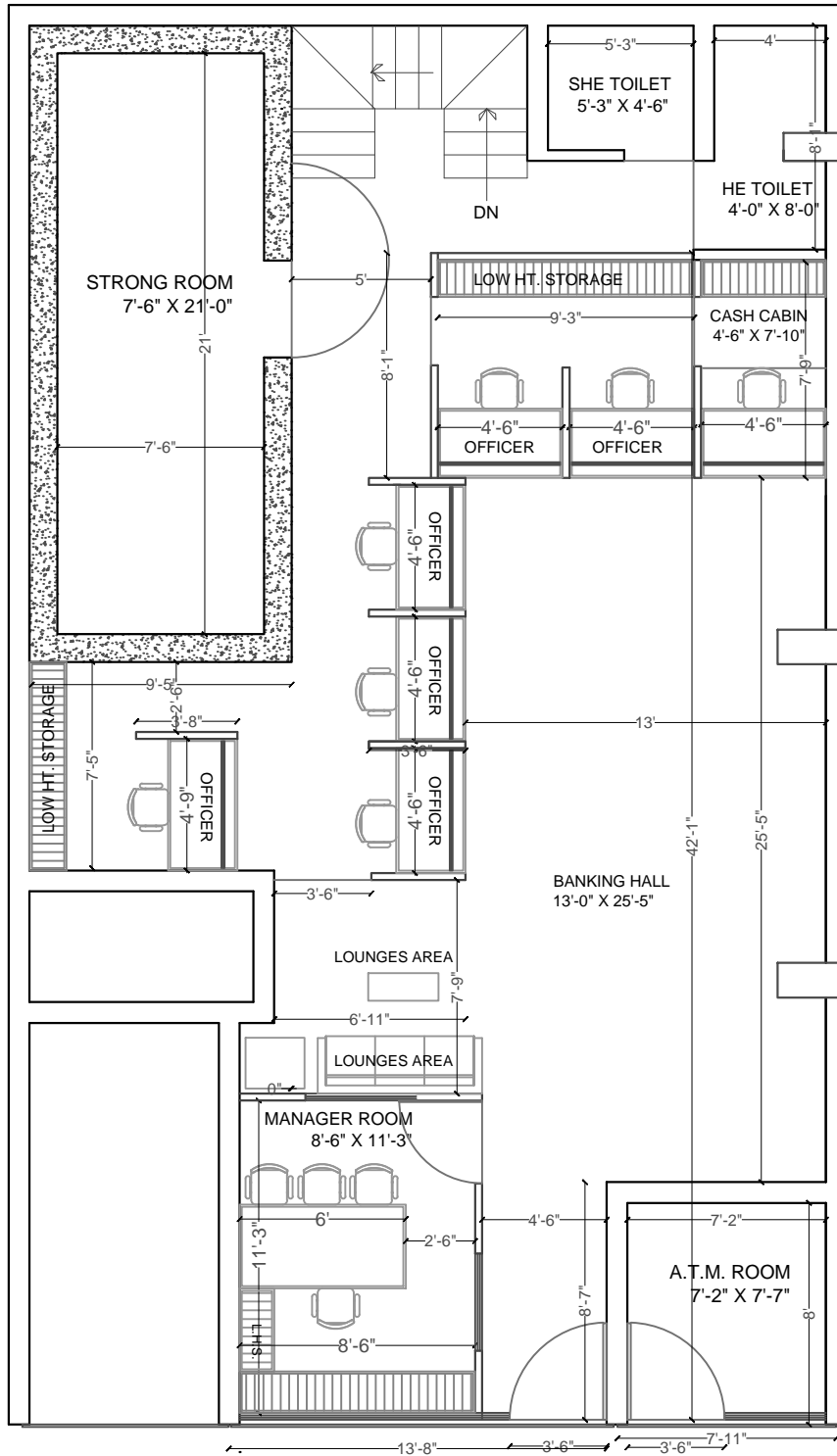
BASEMENT FLOOR
