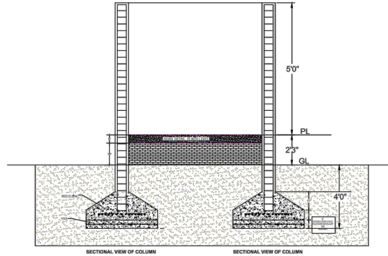
SECTIONAL VIEW (NTS)
